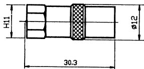
PAL Female-F Male Adaptor
