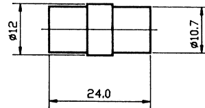
Female-Female Adaptor
