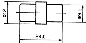
Male-Male Adaptor
