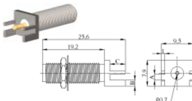
ROUND CONTACT
